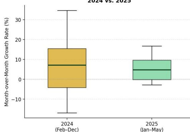
Fig. 5. Narrowing Growth-Rate Volatility: 2024 vs. 2025
