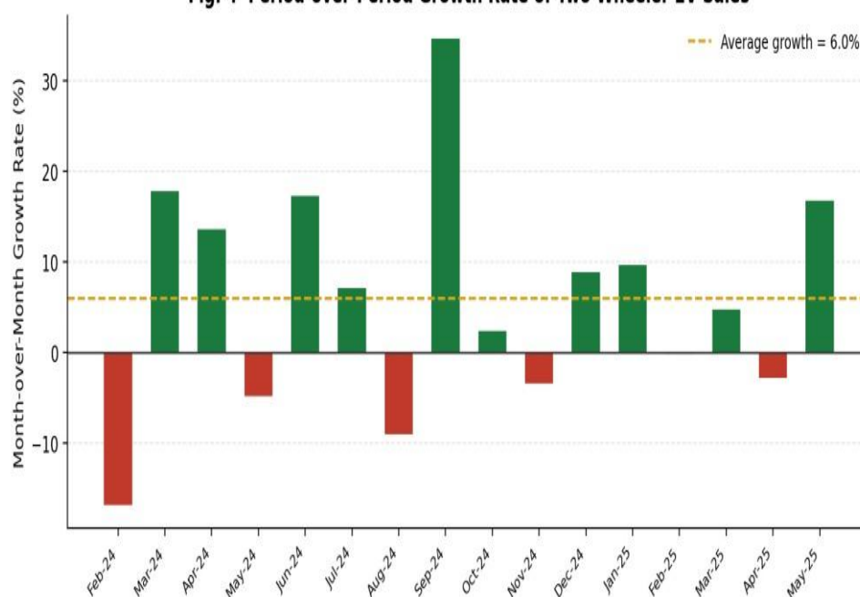
Fig. 4. Month-over-Month Growth Rate of Two-Wheeler EV Sales
