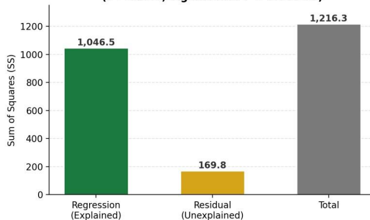
Fig. 2. ANOVA Sum-of-Squares Decomposition — Regression vs. Residual vs. Total
