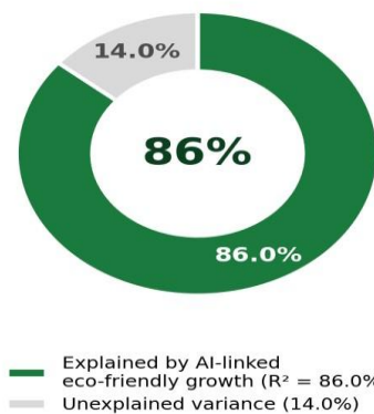
Fig. 1. Explained (86.0%) vs. Unexplained (14.0%) Variance in Two-Wheeler EV Sales
