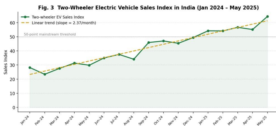
Fig. 3. Two-Wheeler EV Sales Index Trend with Linear Fit
