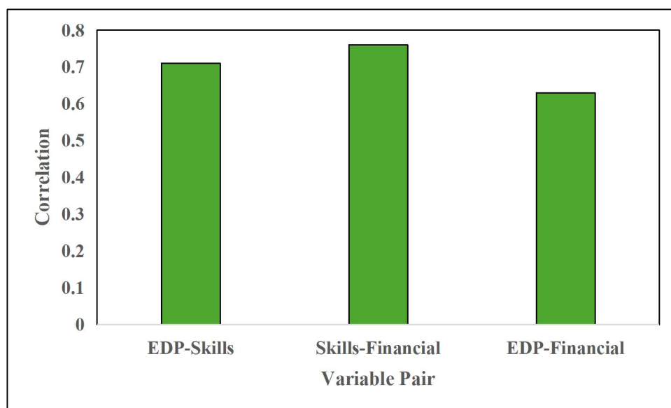
Figure 2. Correlation Between Variables
